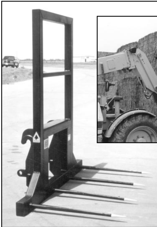
Above: Big Bale Handler.
